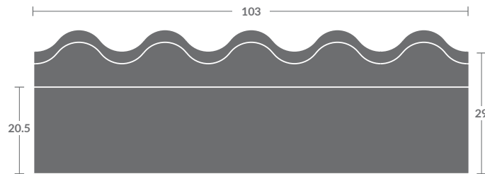
5725-5 Armless Banquette
